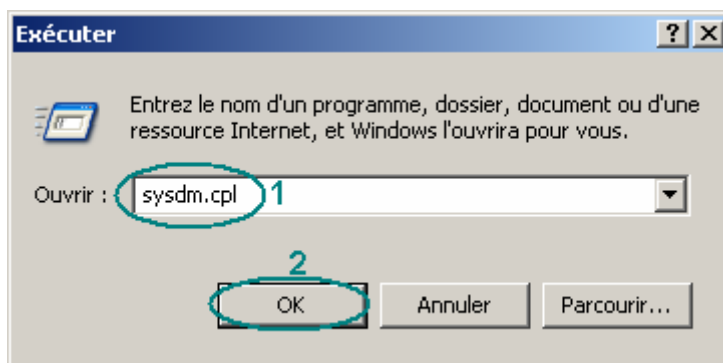
Figure 23 : "sysdm.cpl"
