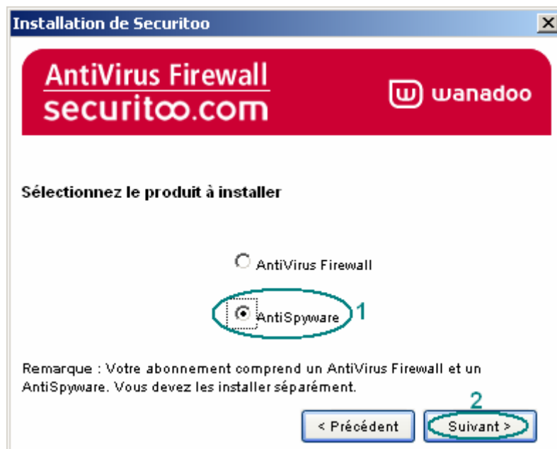
Figure 6 : AntiSpyware
