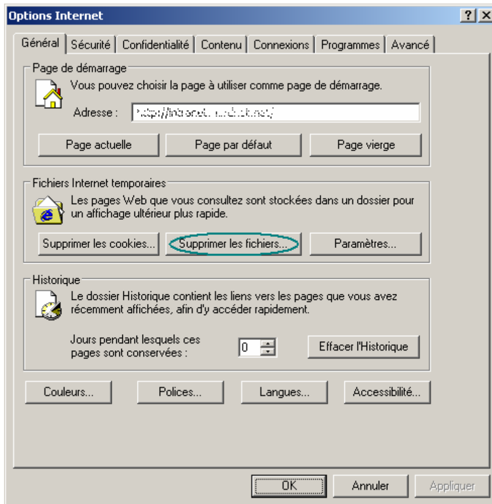
Figure 5 : Options Internet
