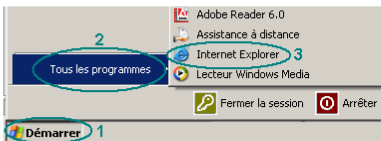
Figure 1 : Lancer IE6
